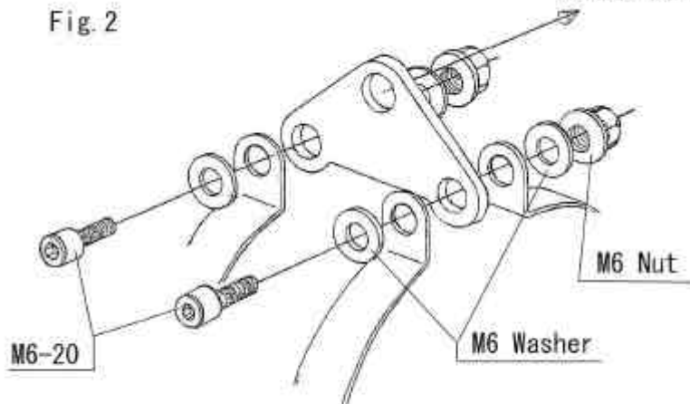
How to attach the silencer band stay
